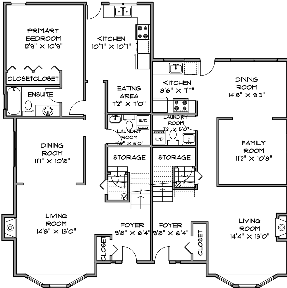
MAIN LEVEL 1072 SQ. FT. SIDE A
