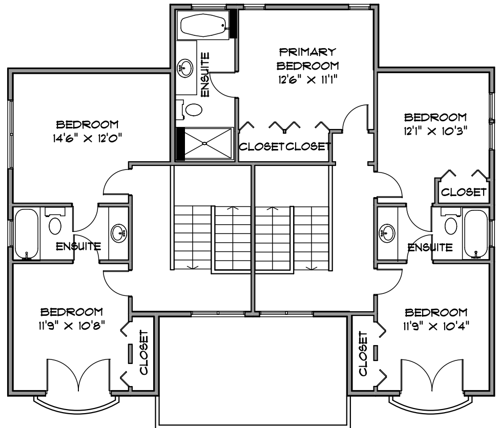
UPPER LEVEL 564 SQ. FT. SIDE A
